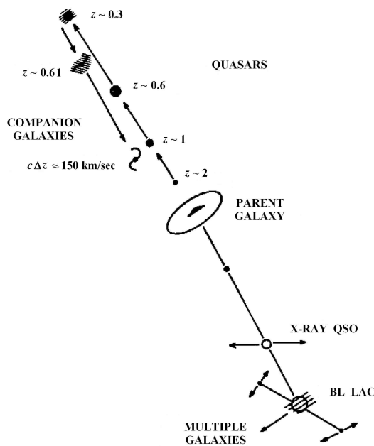
Fig. 2 Schematic representation of quasars and companion galaxies found associated with central galaxies from 1966 to present. The progression of characteristics is empirical but is also required by the variable mass theory of Narlikar and Arp, 1993 [6]
